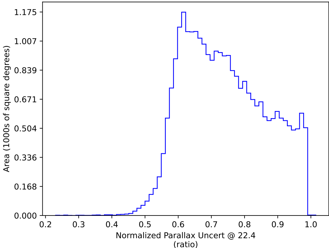
too_elab_heavy_r64_d3_griz_v3.4_10yrs : Normalized Parallax Uncert @ 22.4
