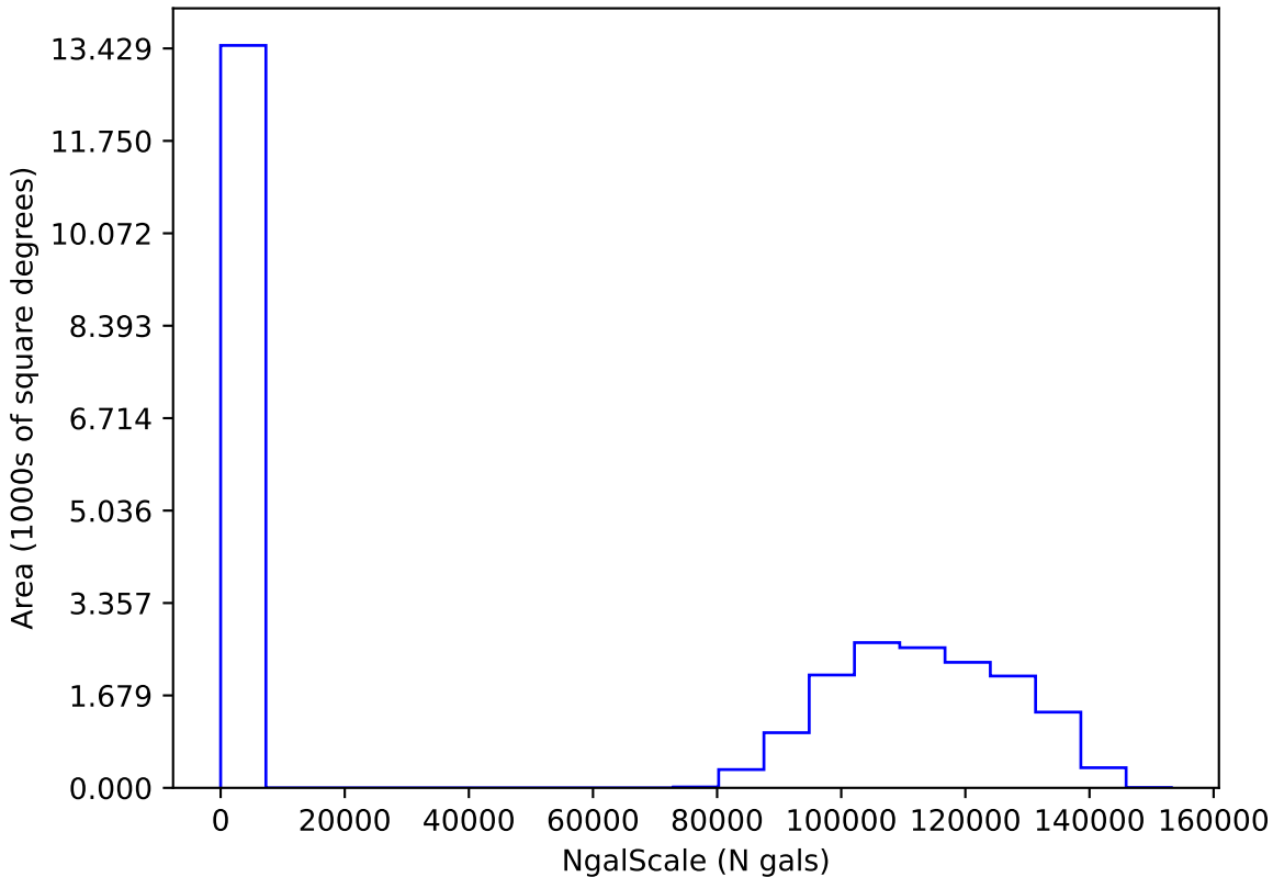
too_elab_heavy_r64_d3_griz_v3.4_10yrs i: NgalScale
