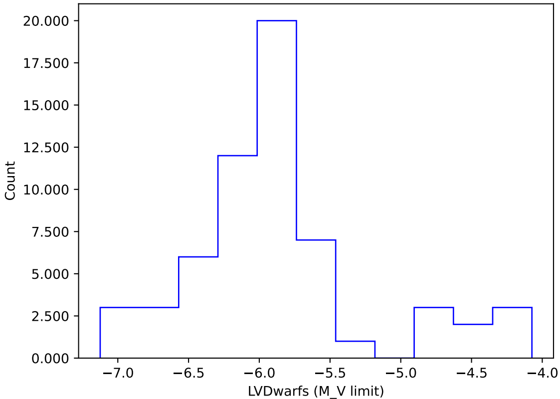
too_elab_heavy_r64_d3_griz_v3.4_10yrs gi: LVDwarfs
