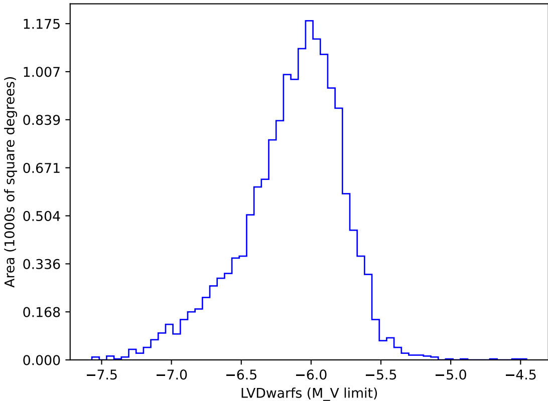
too_elab_heavy_r64_d3_griz_v3.4_10yrs gi: LVDwarfs
