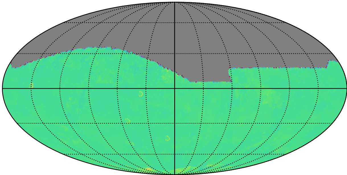
too_elab_heavy_r64_d3_griz_v3.4_10yrs r: Kuiper rotTelPos
