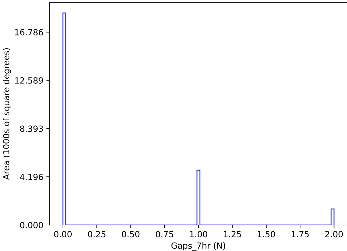
too_elab_heavy_r64_d3_griz_v3.4_10yrs y band: Gaps_7hr
