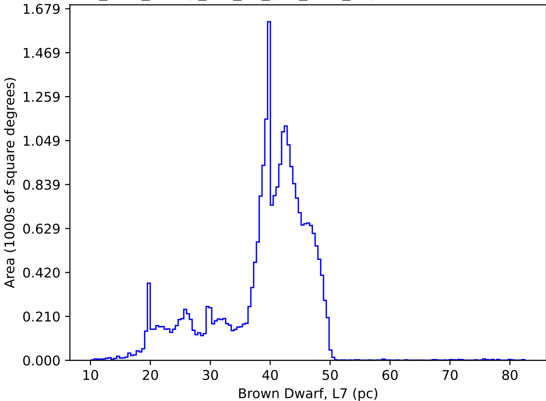
too_elab_heavy_r64_d3_griz_v3.4_10yrs : Brown Dwarf, L7
