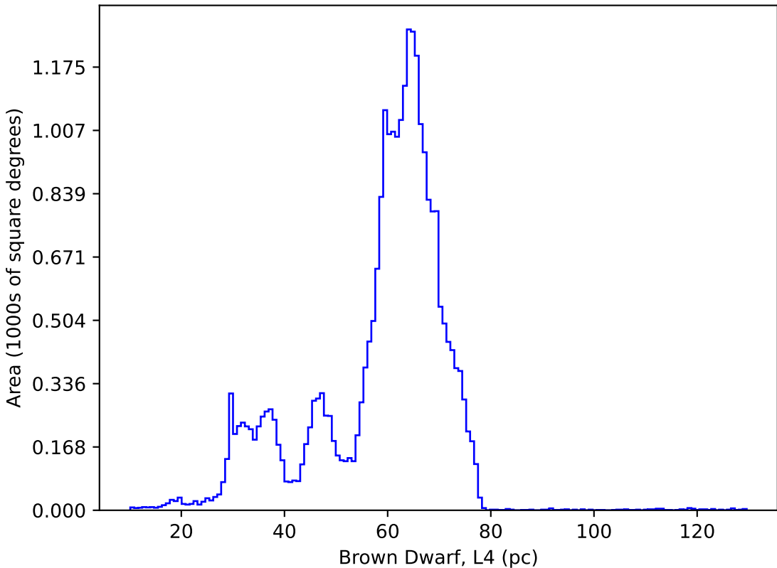
too_elab_heavy_r64_d3_griz_v3.4_10yrs : Brown Dwarf, L4
