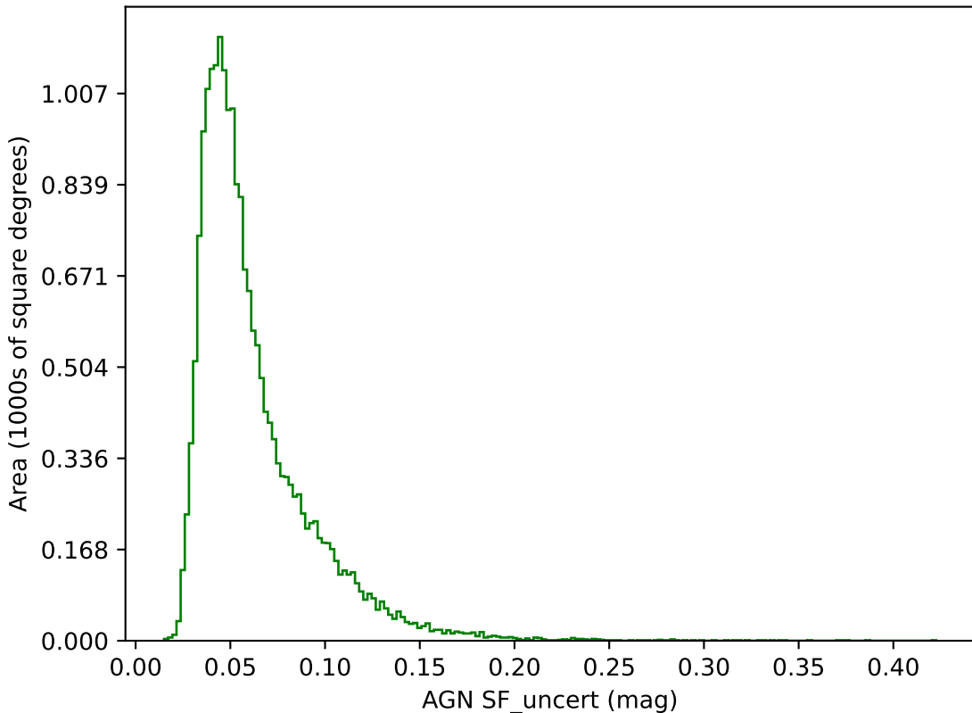
too_elab_heavy_r64_d3_griz_v3.4_10yrs g band: AGN SF_uncert
