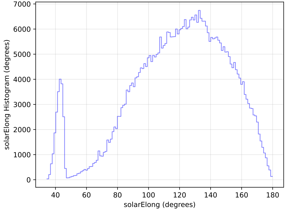
too_elab_heavy_r64_d3_griz_v3.4_10yrs WFD z band: solarElong Histogram
