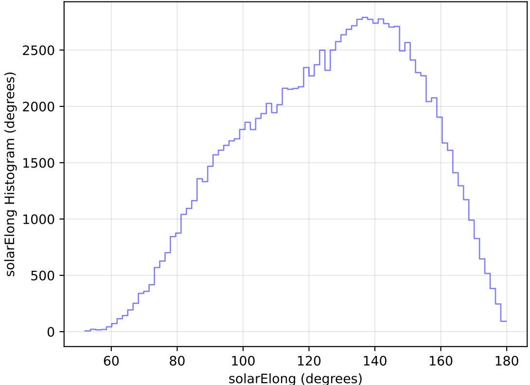
too_elab_heavy_r64_d3_griz_v3.4_10yrs WFD u band: solarElong Histogram
