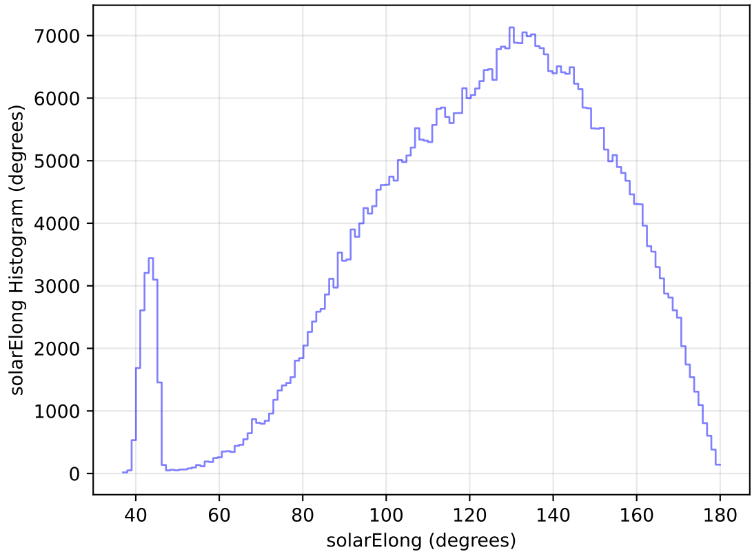
too_elab_heavy_r64_d3_griz_v3.4_10yrs WFD r band: solarElong Histogram
