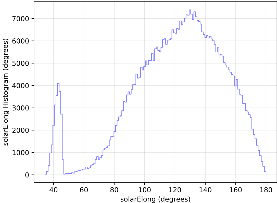
too_elab_heavy_r64_d3_griz_v3.4_10yrs WFD i band: solarElong Histogram
