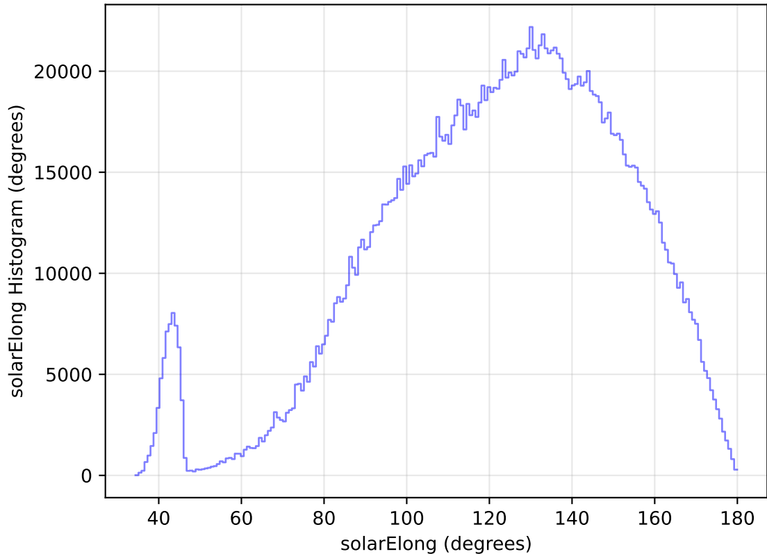
too_elab_heavy_r64_d3_griz_v3.4_10yrs WFD all bands: solarElong Histogram
