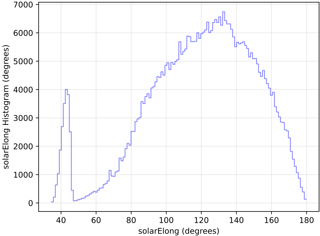
too_elab_heavy_r64_d3_griz_v3.4_10yrs All sky z band: solarElong Histogram
