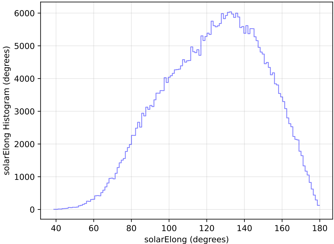
too_elab_heavy_r64_d3_griz_v3.4_10yrs All sky y band: solarElong Histogram
