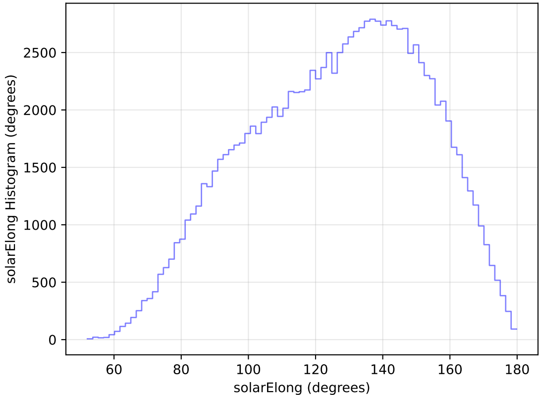
too_elab_heavy_r64_d3_griz_v3.4_10yrs All sky u band: solarElong Histogram
