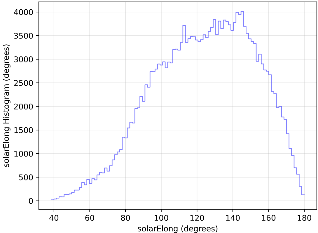
too_elab_heavy_r64_d3_griz_v3.4_10yrs All sky g band: solarElong Histogram
