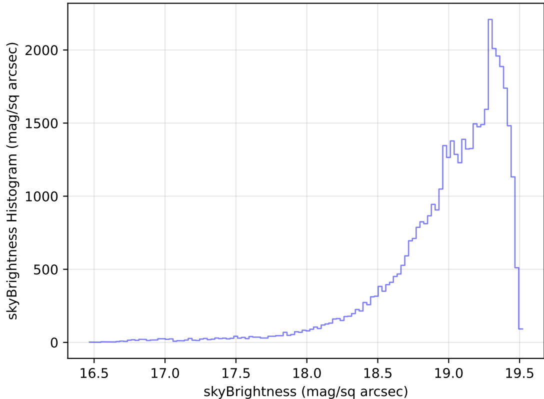
too_elab_heavy_r64_d3_griz_v3.4_10yrs Yr 1 z band: skyBrightness Histogram
