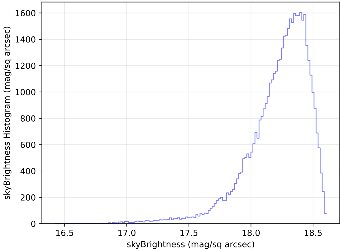
too_elab_heavy_r64_d3_griz_v3.4_10yrs Yr 1 y band: skyBrightness Histogram
