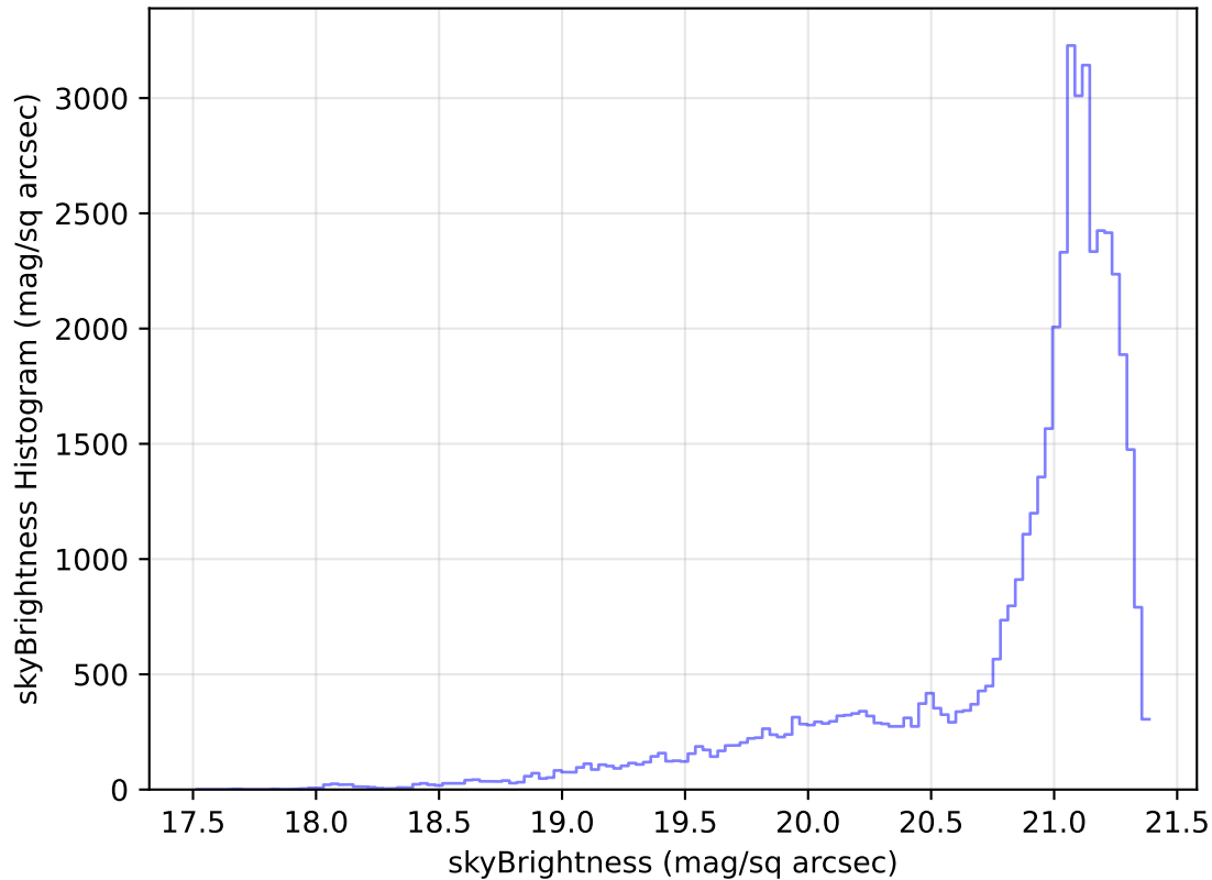
too_elab_heavy_r64_d3_griz_v3.4_10yrs Yr 1 r band: skyBrightness Histogram
