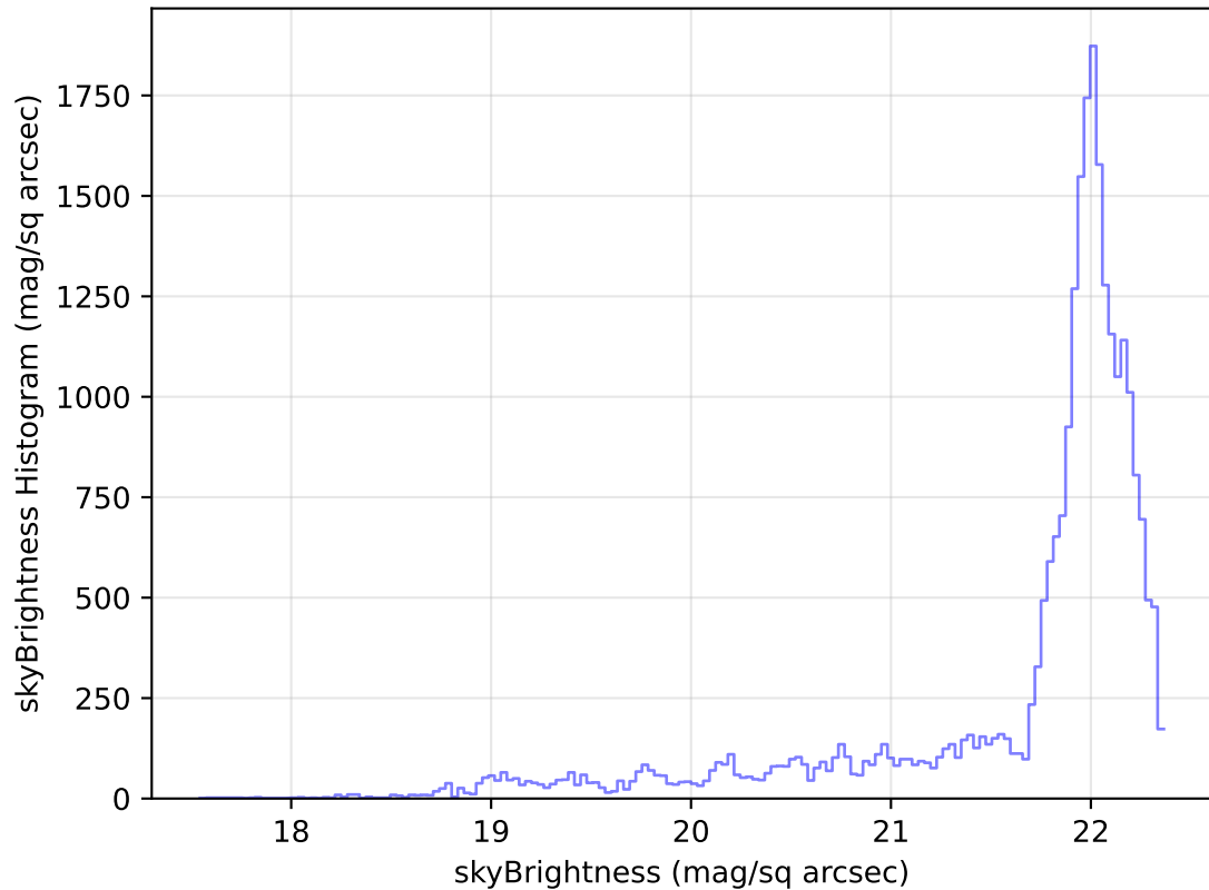
too_elab_heavy_r64_d3_griz_v3.4_10yrs Yr 1 g band: skyBrightness Histogram
