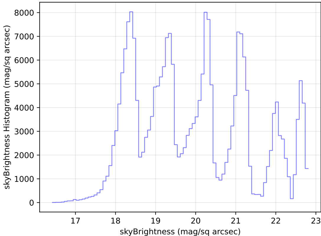
too_elab_heavy_r64_d3_griz_v3.4_10yrs Yr 1 all bands: skyBrightness Histogram
