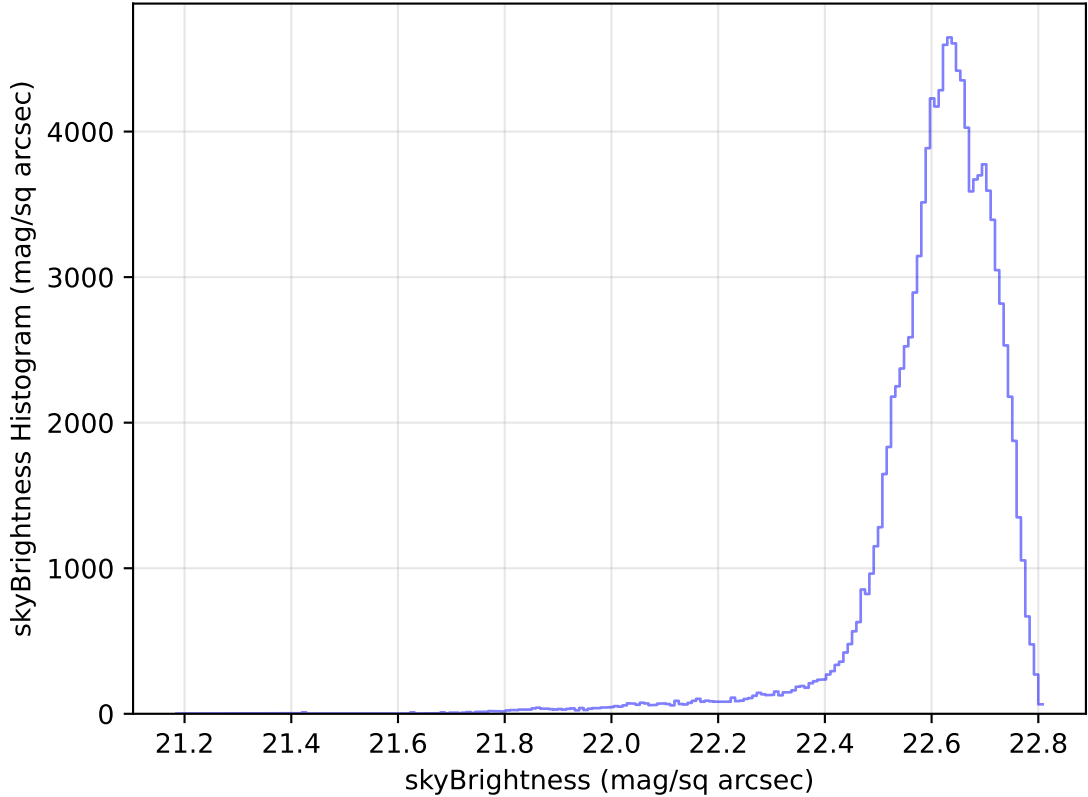
too_elab_heavy_r64_d3_griz_v3.4_10yrs WFD u band: skyBrightness Histogram
