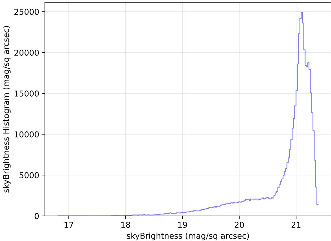
too_elab_heavy_r64_d3_griz_v3.4_10yrs WFD r band: skyBrightness Histogram
