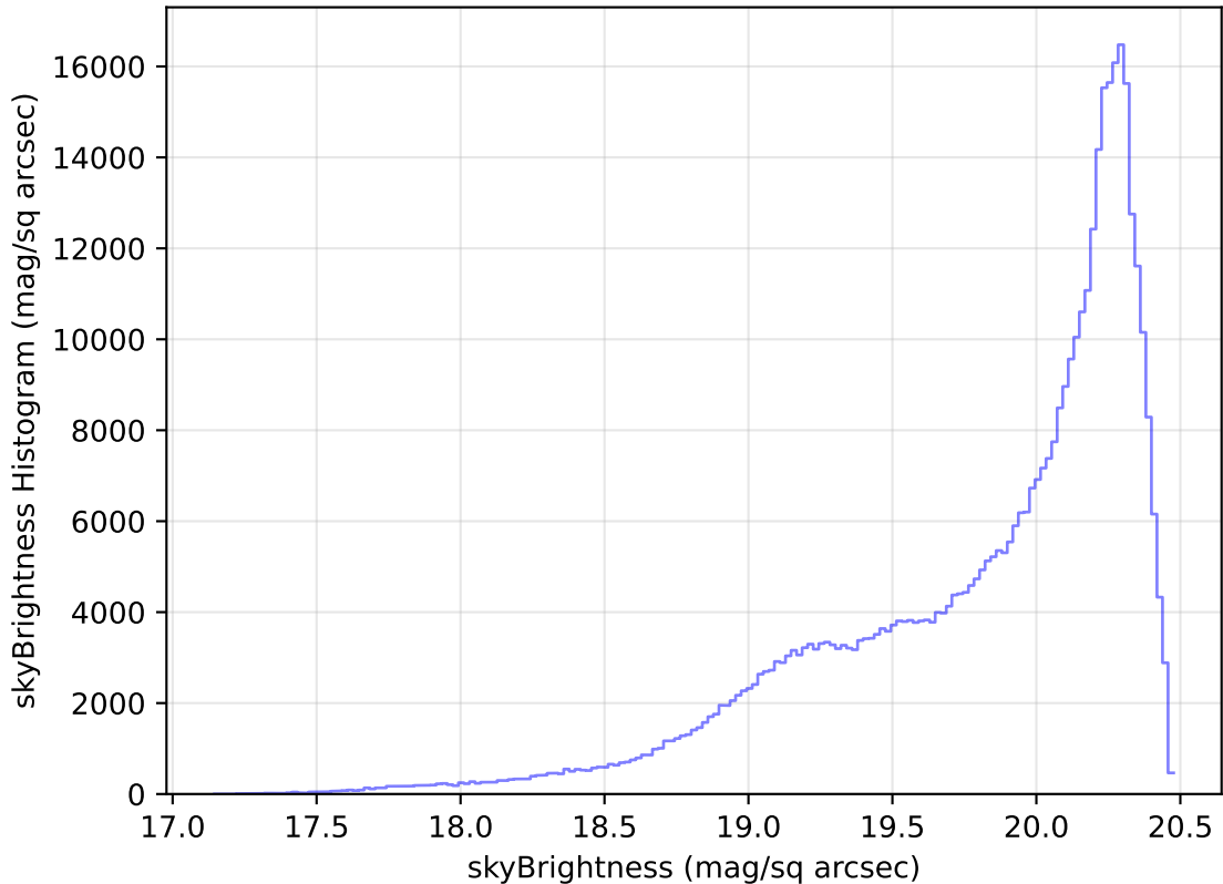
too_elab_heavy_r64_d3_griz_v3.4_10yrs WFD i band: skyBrightness Histogram
