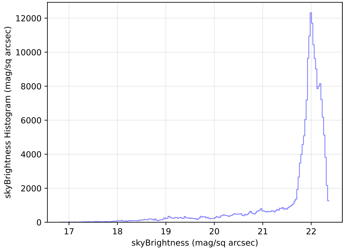
too_elab_heavy_r64_d3_griz_v3.4_10yrs WFD g band: skyBrightness Histogram
