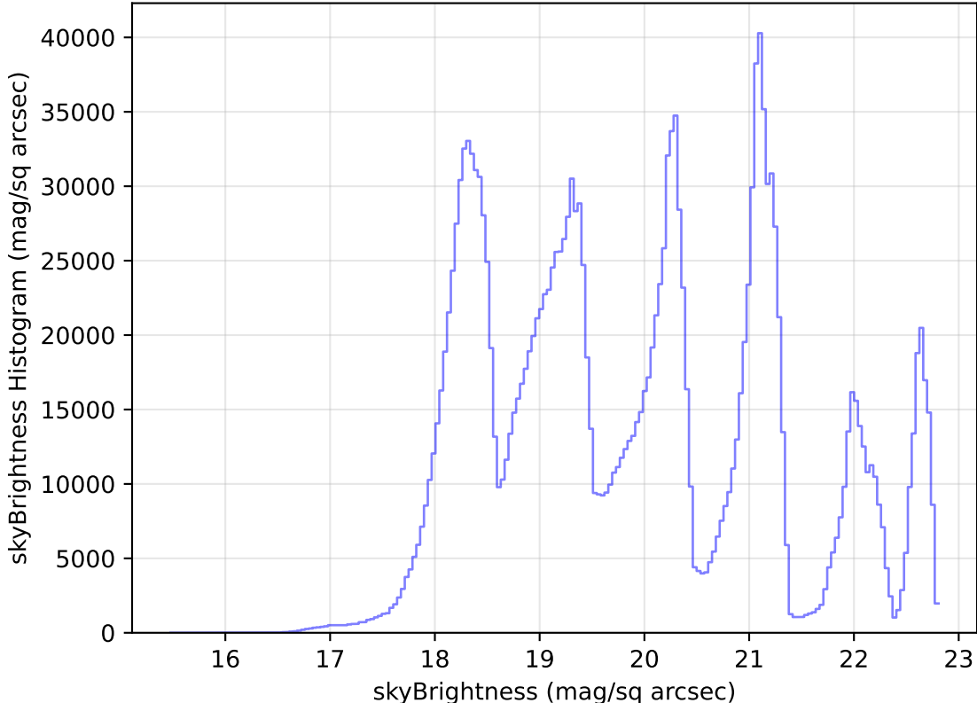
too_elab_heavy_r64_d3_griz_v3.4_10yrs WFD all bands: skyBrightness Histogram
