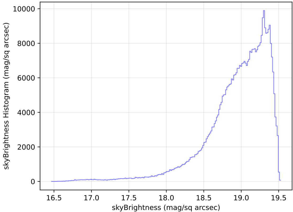
too_elab_heavy_r64_d3_griz_v3.4_10yrs All sky z band: skyBrightness Histogram
