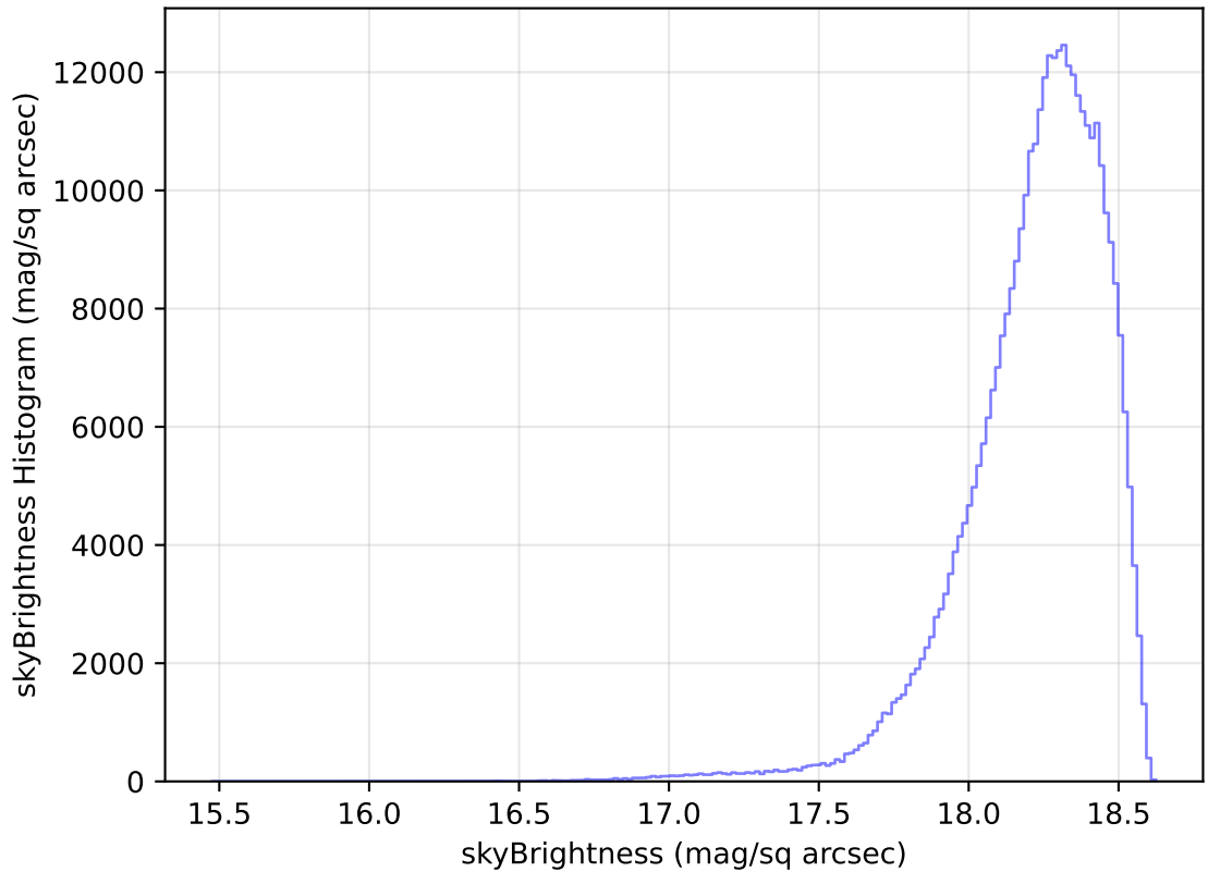
too_elab_heavy_r64_d3_griz_v3.4_10yrs All sky y band: skyBrightness Histogram
