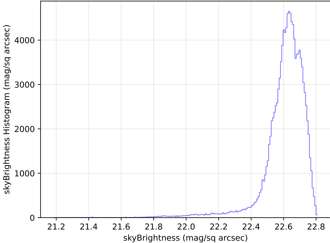
too_elab_heavy_r64_d3_griz_v3.4_10yrs All sky u band: skyBrightness Histogram
