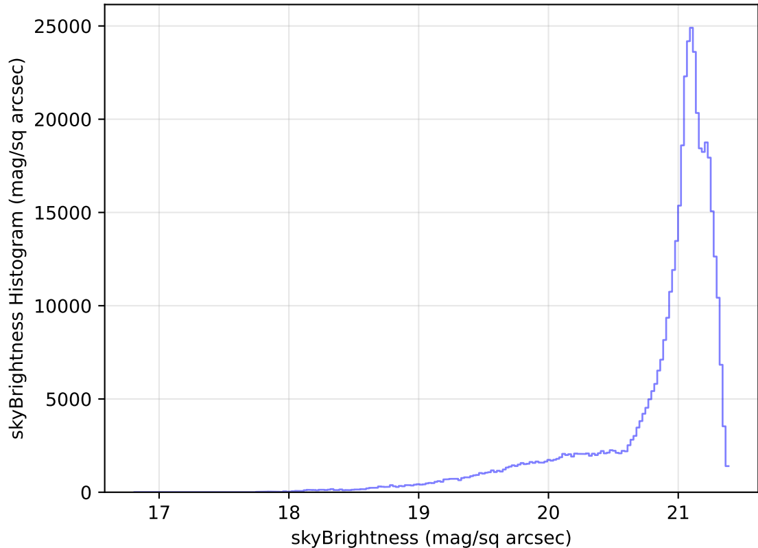
too_elab_heavy_r64_d3_griz_v3.4_10yrs All sky r band: skyBrightness Histogram
