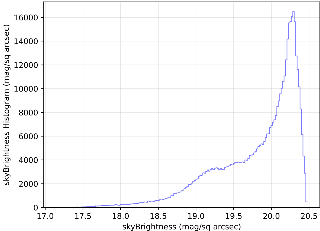
too_elab_heavy_r64_d3_griz_v3.4_10yrs All sky i band: skyBrightness Histogram
