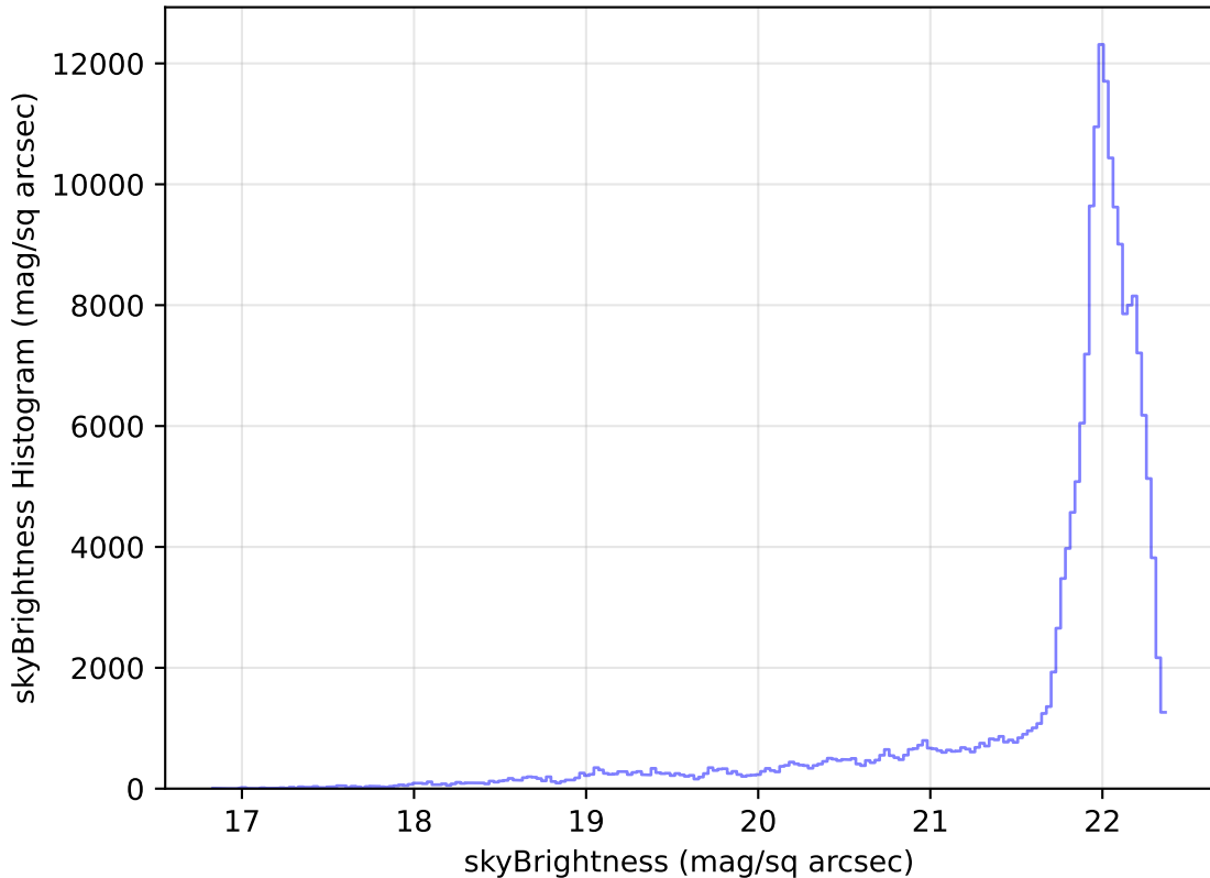
too_elab_heavy_r64_d3_griz_v3.4_10yrs All sky g band: skyBrightness Histogram
