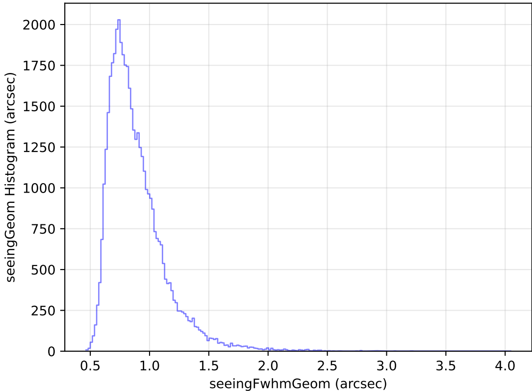
too_elab_heavy_r64_d3_griz_v3.4_10yrs Yr 1 z band: seeingGeom Histogram
