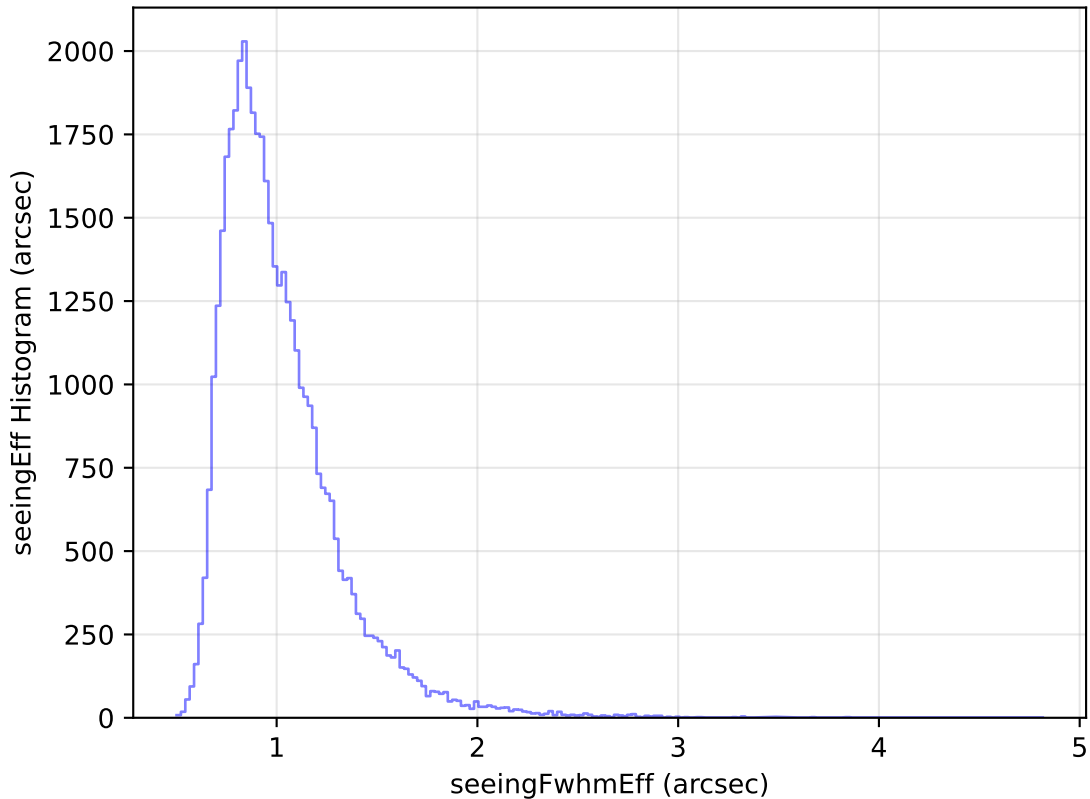
too_elab_heavy_r64_d3_griz_v3.4_10yrs Yr 1 z band: seeingEff Histogram
