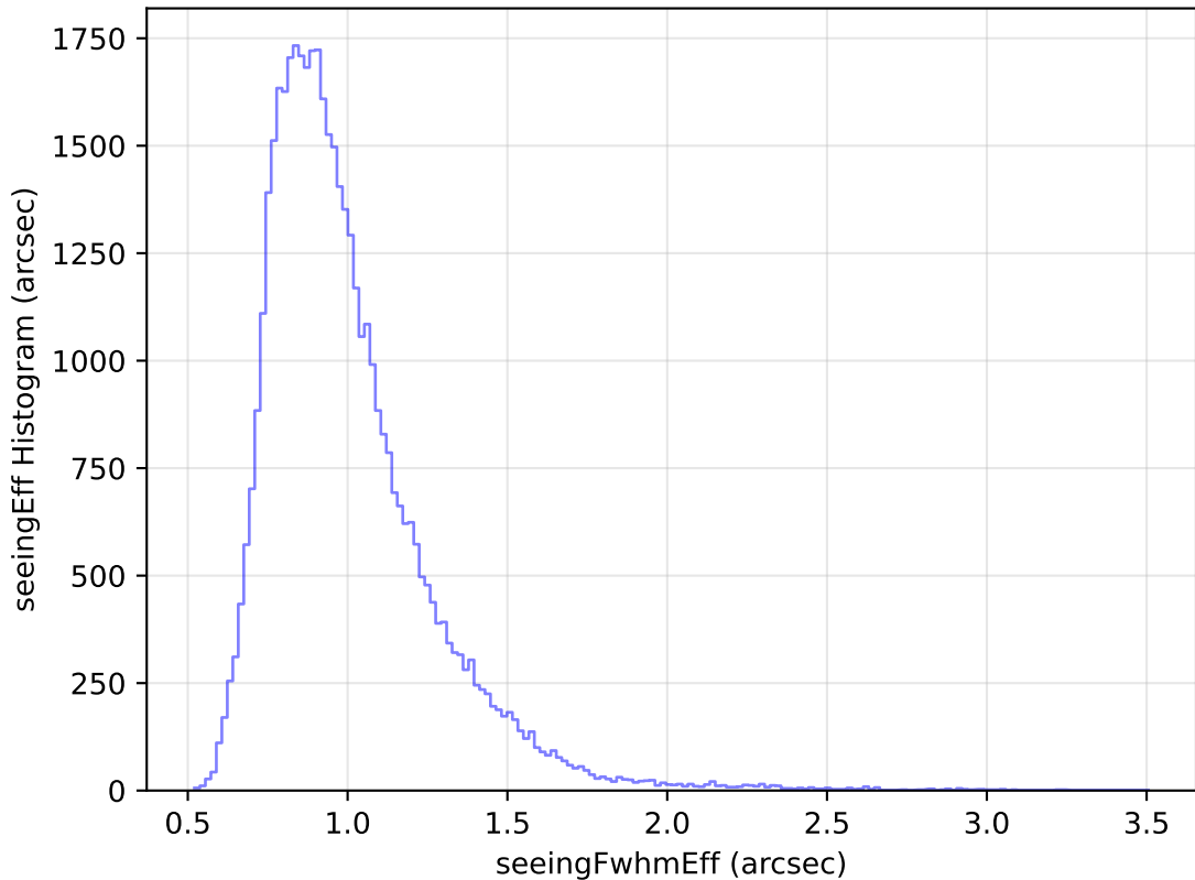
too_elab_heavy_r64_d3_griz_v3.4_10yrs Yr 1 y band: seeingEff Histogram
