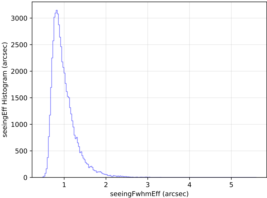
too_elab_heavy_r64_d3_griz_v3.4_10yrs Yr 1 i band: seeingEff Histogram
