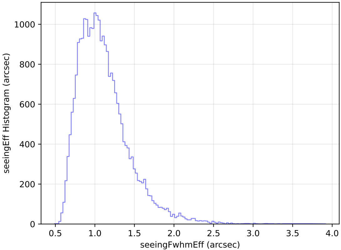
too_elab_heavy_r64_d3_griz_v3.4_10yrs Yr 1 g band: seeingEff Histogram
