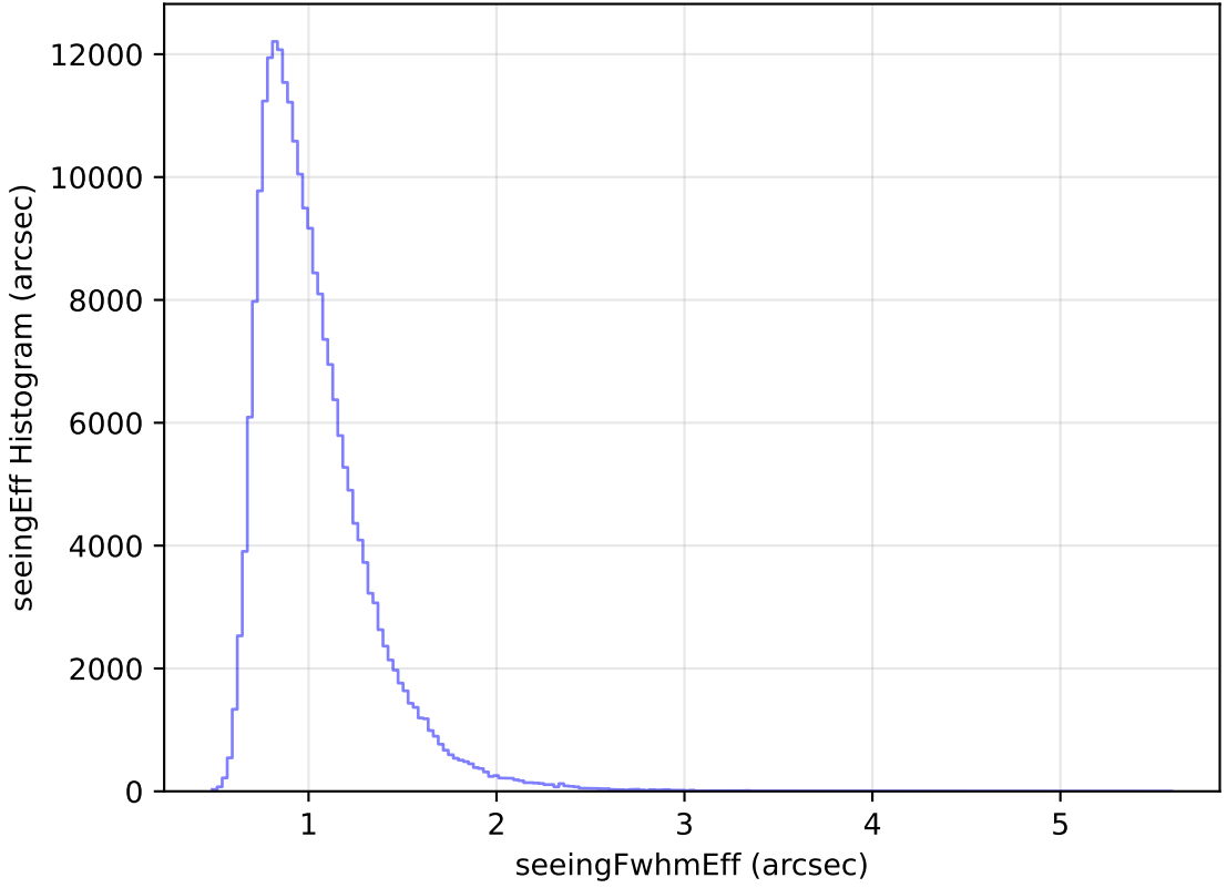
too_elab_heavy_r64_d3_griz_v3.4_10yrs Yr 1 all bands: seeingEff Histogram
