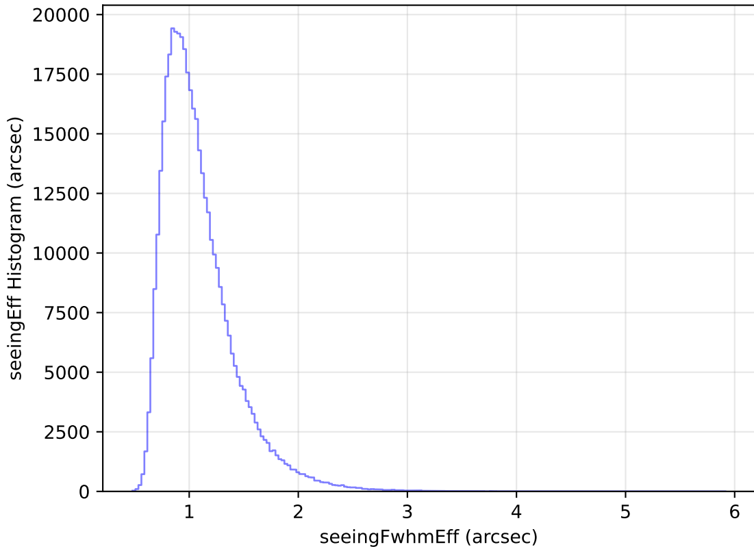
too_elab_heavy_r64_d3_griz_v3.4_10yrs WFD z band: seeingEff Histogram
