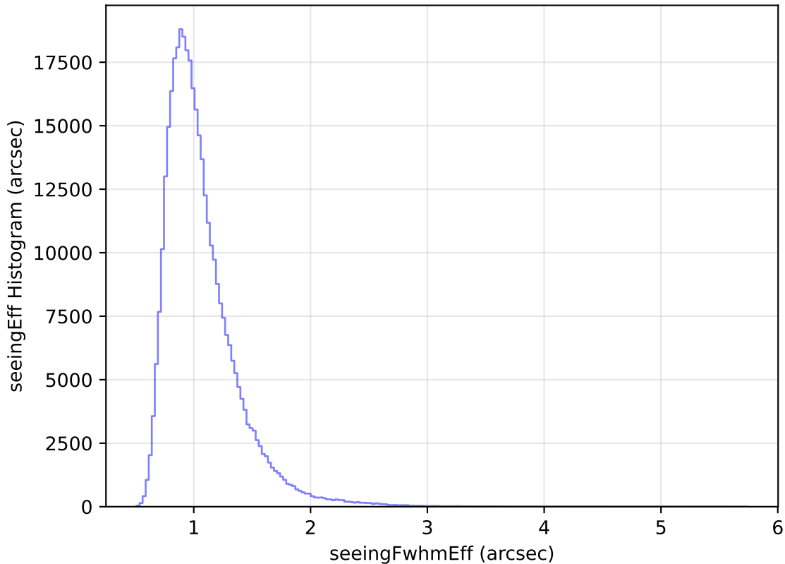
too_elab_heavy_r64_d3_griz_v3.4_10yrs WFD y band: seeingEff Histogram
