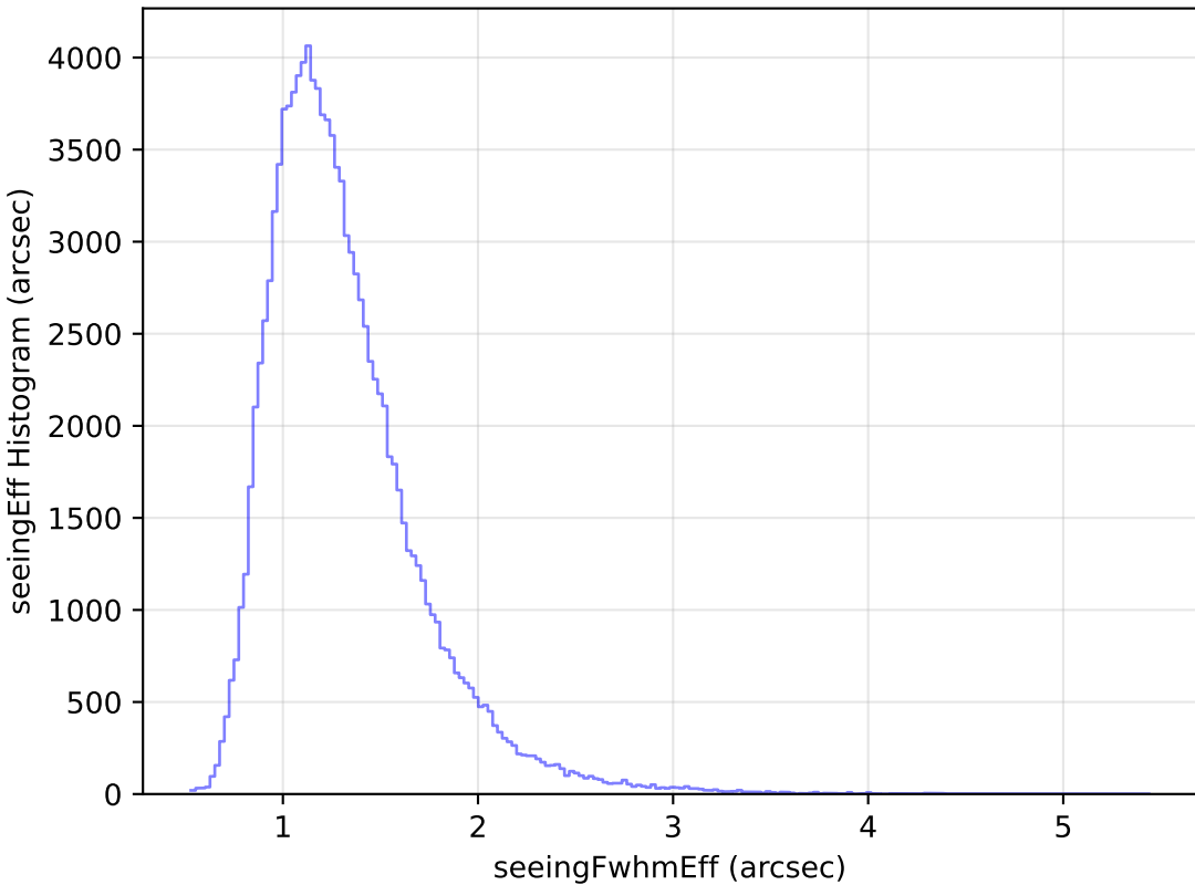
too_elab_heavy_r64_d3_griz_v3.4_10yrs WFD u band: seeingEff Histogram
