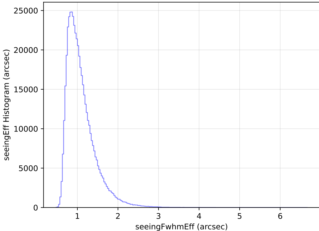
too_elab_heavy_r64_d3_griz_v3.4_10yrs WFD i band: seeingEff Histogram
