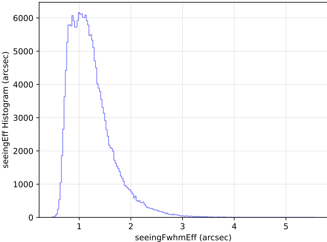
too_elab_heavy_r64_d3_griz_v3.4_10yrs WFD g band: seeingEff Histogram
