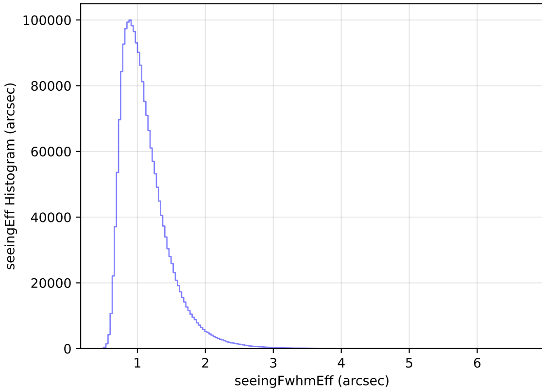
too_elab_heavy_r64_d3_griz_v3.4_10yrs WFD all bands: seeingEff Histogram
