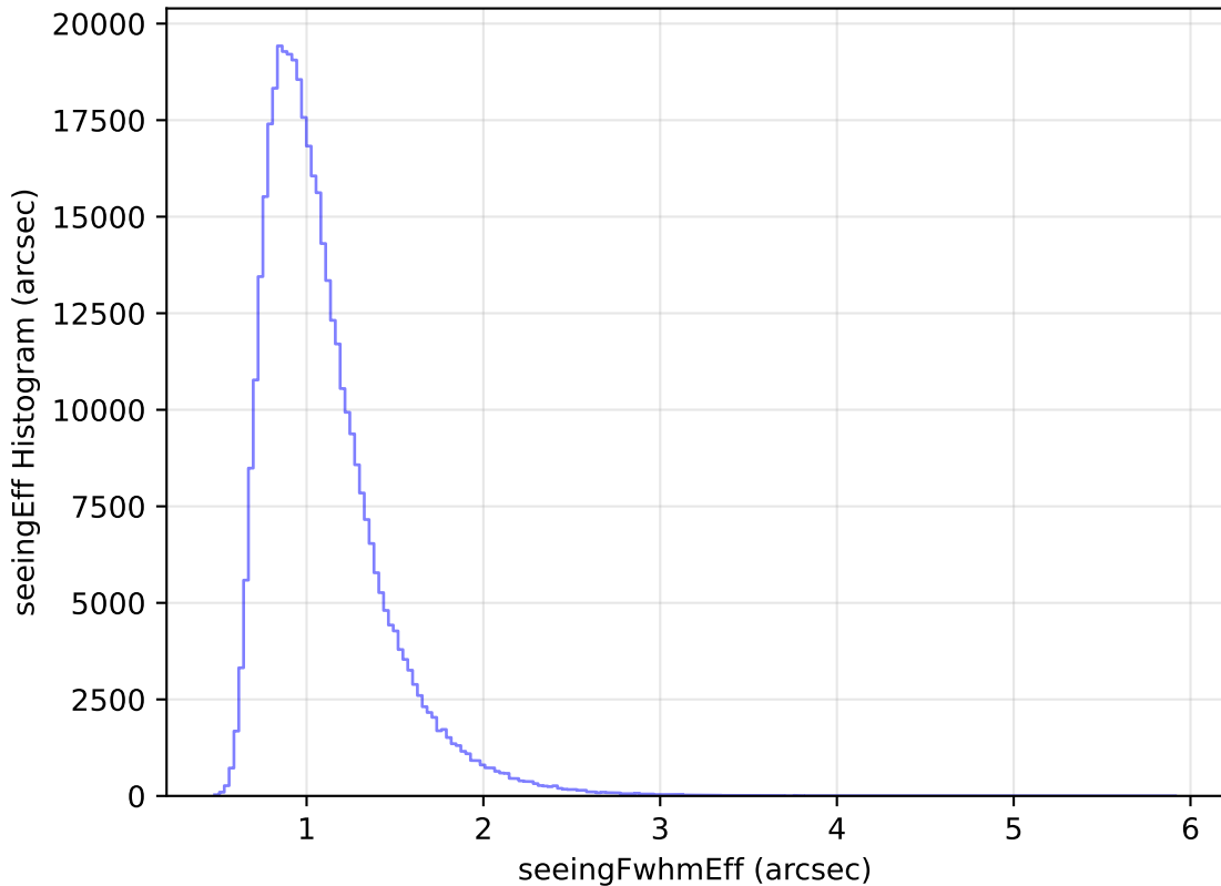
too_elab_heavy_r64_d3_griz_v3.4_10yrs All sky z band: seeingEff Histogram
