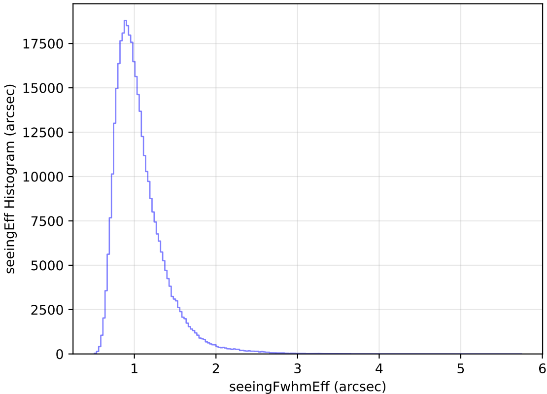
too_elab_heavy_r64_d3_griz_v3.4_10yrs All sky y band: seeingEff Histogram
