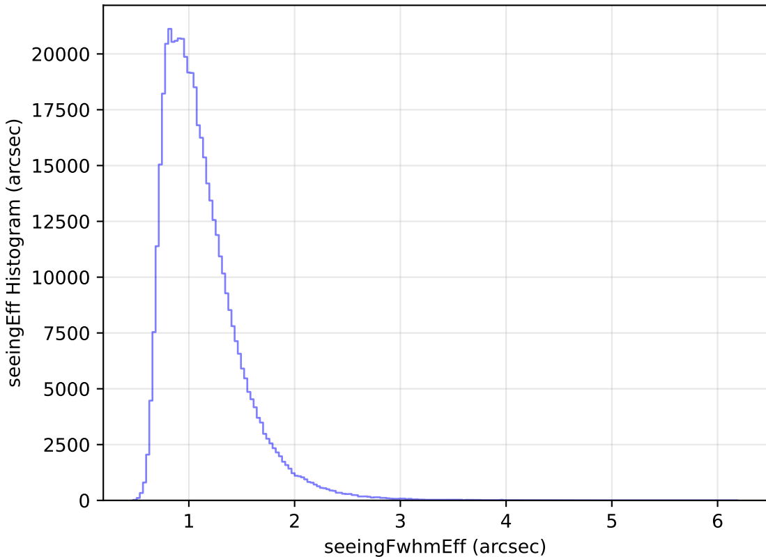
too_elab_heavy_r64_d3_griz_v3.4_10yrs All sky r band: seeingEff Histogram
