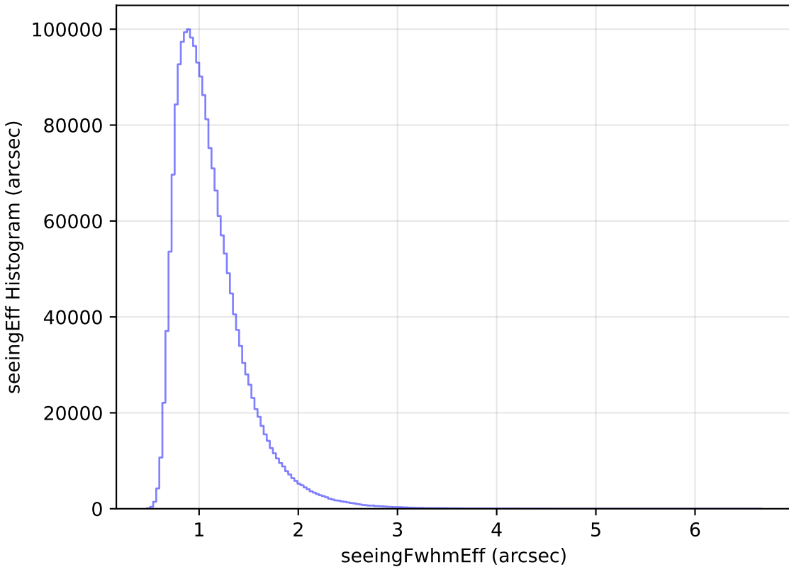
too_elab_heavy_r64_d3_griz_v3.4_10yrs All sky all bands: seeingEff Histogram
